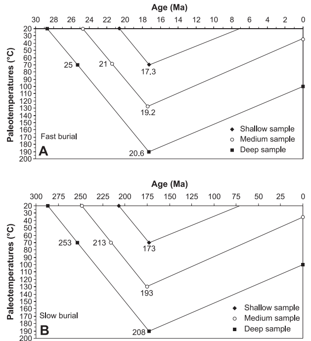
FIGURE 5. Thermal history curves for 3 depths from a single well in two hypothetical basins: (A) fast burial; (B) slow burial. For a given well, each of the three samples was buried to reach the onset of illitization (70 °C) at different times (shown in the figures), but reached their maximum paleotemperatures (end of illitization) at the same time. These curves are used to model the K-Ar age of the total diagenetically formed illite at the end of illitization (“the mixed diagenetic age” indicated by the bold numbers in each figure) using the decaying nucleation rate mechanism (option 3 in GALOPER). The shallow sample just reached the 70 °C isotherm, thus its onset age equals its end of illitization age. In the case of fast burial (A), the absolute difference in the final calculated ages between the shallow and the deep sample is small (3.3 Ma = “punctuated diagenesis”), while it is large for the slow burial case (B, 35 Ma). This figure illustrates how aspects of the burial history can be revealed from a set of K-Ar dates obtained from varying depths of a single well.
