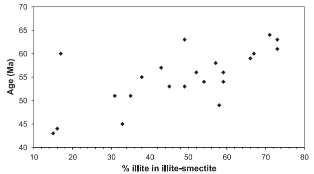
FIGURE 6. Data of Elliot et al. (1991) for illite-smectites from bentonites from the Denver Basin, documenting the K-Ar mixed age trend predicted by Figure 5B. The %I in illite-smectite is a proxy for the maximum paleotemperatures, and ca. 20 Ma difference in age is indicative of a slow burial scenario (Fig. 5B).
