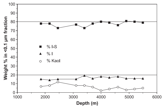
FIGURE 9. Measured (% kaolinite) and calculated (% illite-smectite and % illite) composition of <0.1 \mu\text{m} fraction from the shales of CWRU 6 well, used in the model presented in Figure 8.
