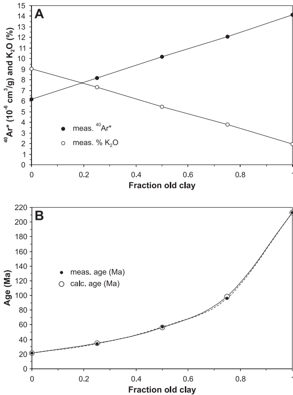
FIGURE 7. K-Ar data for artificial mixtures of a 22 Ma illite and a 213 Ma illite-smectite, verifying the theoretical approach to modeling mixtures used in this study (Środoń 1999b). Measured K 2 O (%) and radiogenic 40 Ar* values (in 10 -6 cm 3 /g) are shown in Figure 7A, and measured and calculated mixed ages in 7B.
