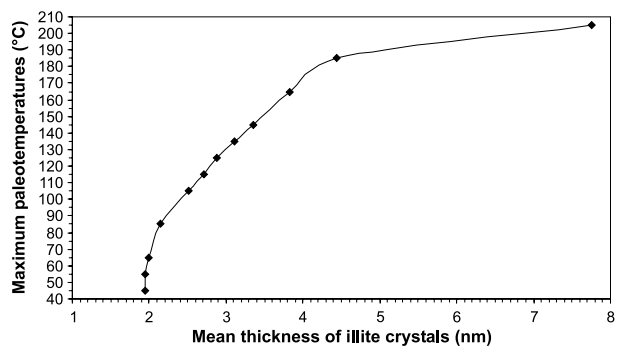
FIGURE 1. Relation between the mean thickness of illite fundamental particles and the maximum paleotemperatures, established by applying Equations 1–3 to Figure 3 of Sucha et al. (1993). This relation is used to model the mixed ages presented in Figure 2.
