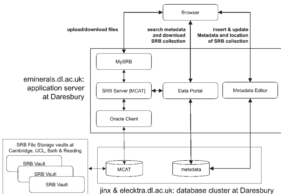
Figure 2. The structure of the data component of the eMinerals minigrid.
