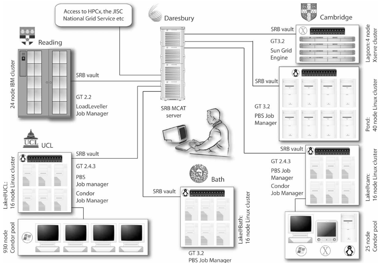
Figure 1. The structure of the eMinerals minigrid. The diagram is organised to highlight the middleware tools as the core of the infrastructure.
