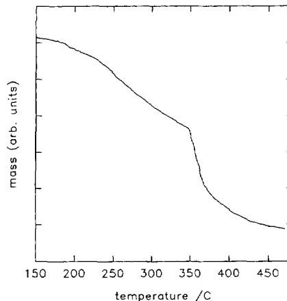
Fig 3. Mass vs temperature curve for a CRTA experiment (the change in slope is due to the change in the decomposition rate).
