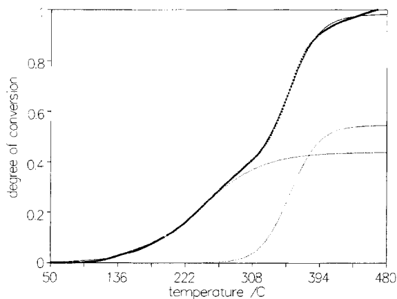
Fig. 1. Variation with temperature of the conversion degree \alpha corresponding to the deintercalation reaction (* experimental points, .... suggested decomposition steps).
